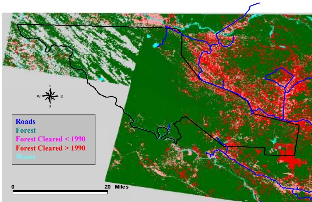
Figure 2. Composite Satellite image of the SLNP indicating deforestation prior to 1990 and from 1990 to 1999.
