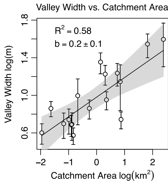
Figure 9. Plot of incised valley floor width versus catchment area. Error bars represent 1 standard deviation of width values derived from valley floor polygons digitized from SPOT5 imagery and analyzed according to the method of Fisher et al. [2013]. Valley width, W , increases with catchment size, A , as W \propto A^b , with exponent b = 0.2 \pm 0.1 .
