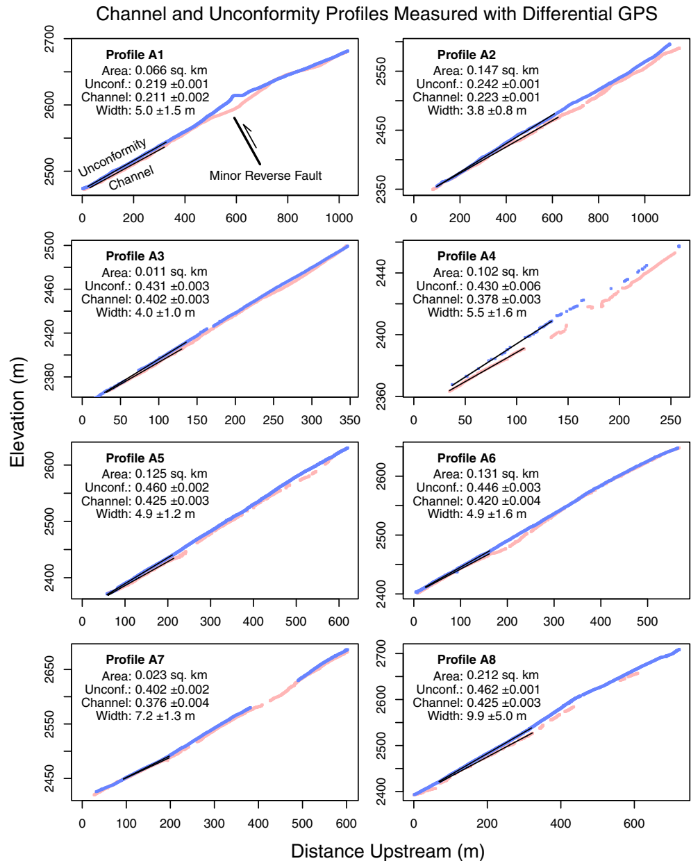
Figure 5. Channel and unconformity surveys for channels A1–A8. Upstream catchment area, best-fitting slopes ( \pm 95\% confidence) for channel outlet and unconformity and valley width ( \pm 1\sigma ) shown for channel. Unconformity points blue and channel points red. Note the locally deeper channel incision in profile A1 across a minor reverse fault that offsets the unconformity surface.
