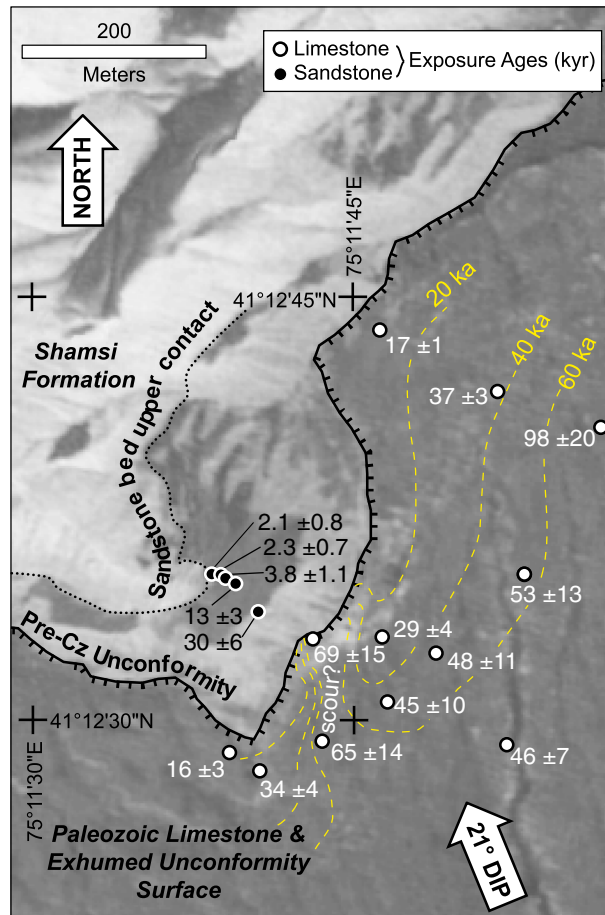
Figure 10. 36 Cl exposure ages from Baybeiche cuesta (see Figure 4 for location) show progressive stripping of Cenozoic cover strata, revealing resistant Paleozoic limestone beneath the unconformity. Ages shown here calculated assuming a surface-lowering rate of 7.5 mm/kyr. Background is orthorectified SPOT-5 panchromatic image. Yellow exposure age contours show interpreted positions through time of the unconformity between Cenozoic and Paleozoic rocks. Anomalous old age from Paleozoic limestone near contact with Cenozoic strata may be due to localized channel scour that prematurely exposed the limestone. Ages are also shown for exposure of a resistant sandstone bed within the lowermost Shamsi formation. These ages are consistent with the overall rate of exposure of the limestone, below, and together the suite of data support an overall steady state northward retreat of the cuesta.
