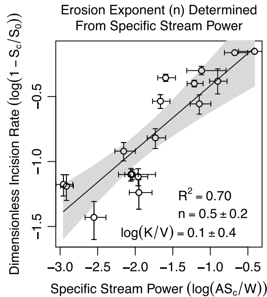
Figure 12. Plot of dimensionless erosion rate, l , versus specific stream power calculated for channels with valley width data. Least-squares regression slope indicates the exponent, n = 0.5 \pm 0.2 , for the relationship of erosion rate to specific stream power. Error bars and shaded areas show 95% confidence of values and regression lines.
