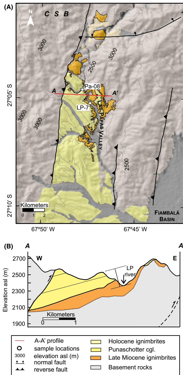
Fig. 2 (A) Geological map of the middle and southern part of the Las Papas valley showing the distribution of the Las Papas Ignimbrites and Punaschotter conglomerates, and sample locations. (B) AA' cross profile illustrates the relationship between the Las Papas Ignimbrites and paleotopography. See the bar tilted 15° to the SW, indicating the (minimum) measured thickness of the Las Papas Ignimbrites.
