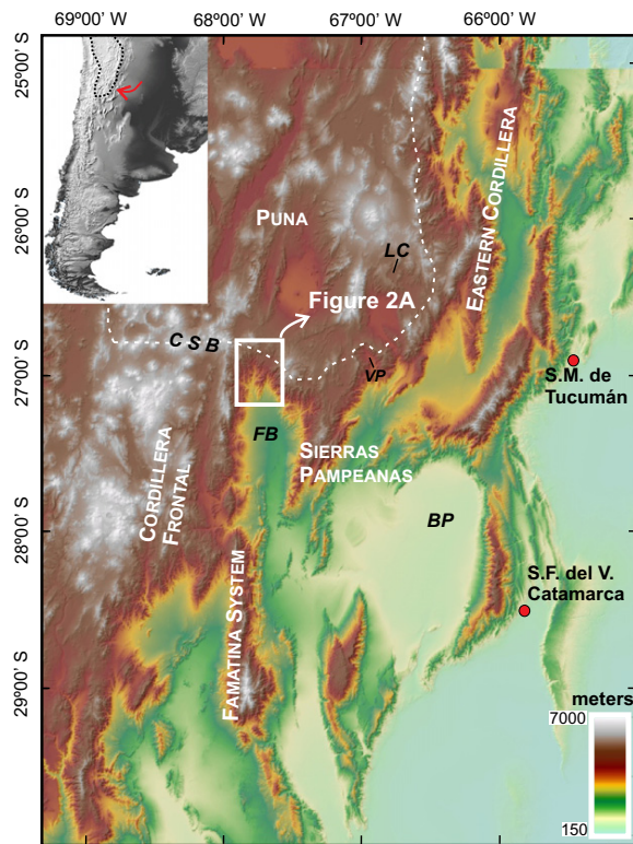
Fig. 1 Digital Elevation Model (DEM) of northwest Argentina showing the location of the Puna plateau. White box shows location of study area. CSB, Cordillera de San Buenaventura; FB, Fiambalá Basin; BP, Bolsón de Pipanaco; VP, Vicuña Pampa; LC, Luigo Caldera.
