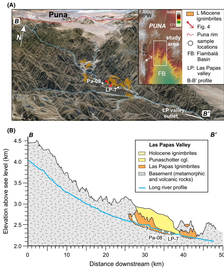
Fig. 3 (A) Three-dimensional perspective view of the outcrop pattern of the late Miocene ignimbrites that filled local paleotopography across the southern Puna plateau margin. (B) Long river profile of the Las Papas River with the sample locations and the units exposed along the valley.
