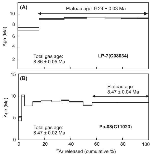
Fig. 5 ^{40}\text{Ar}/^{39}\text{Ar} step-heating experiment results and plateau ages of Las Papas Ignimbrites. (A) Sample LP-7 ( 27^{\circ}04'52.4''\text{S} , 67^{\circ}47'21.4''\text{W} ); (B) Sample Pa-08 ( 27^{\circ}04'11.6''\text{S} , 67^{\circ}47'48.8''\text{W} ).
