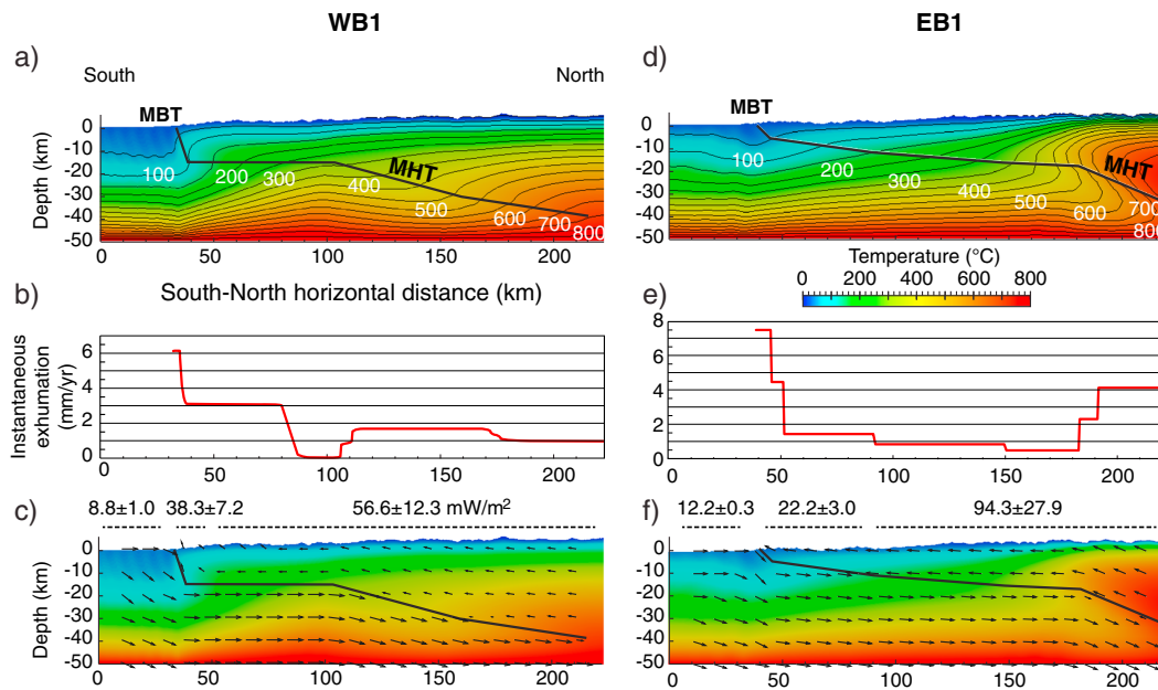
Figure 10. Thermal field and instantaneous exhumation rates for single-stage inversions in western and eastern Bhutan. Cross sections showing MHT geometry with thermal field, instantaneous exhumation rates, and velocity vectors for the (a–c) western (WB1) and (d–f) eastern (EB1) transects. Values of the predicted mean heat flow ( \text{mW/m}^2 ) are provided in Figures 10c and 10f for the foreland, LHS, and GHS units.
